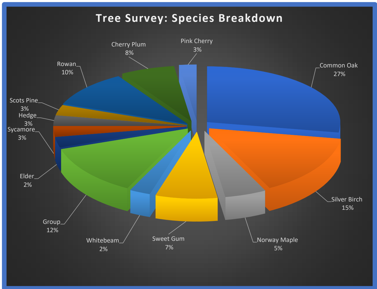
Figure 7 Species Distribution
