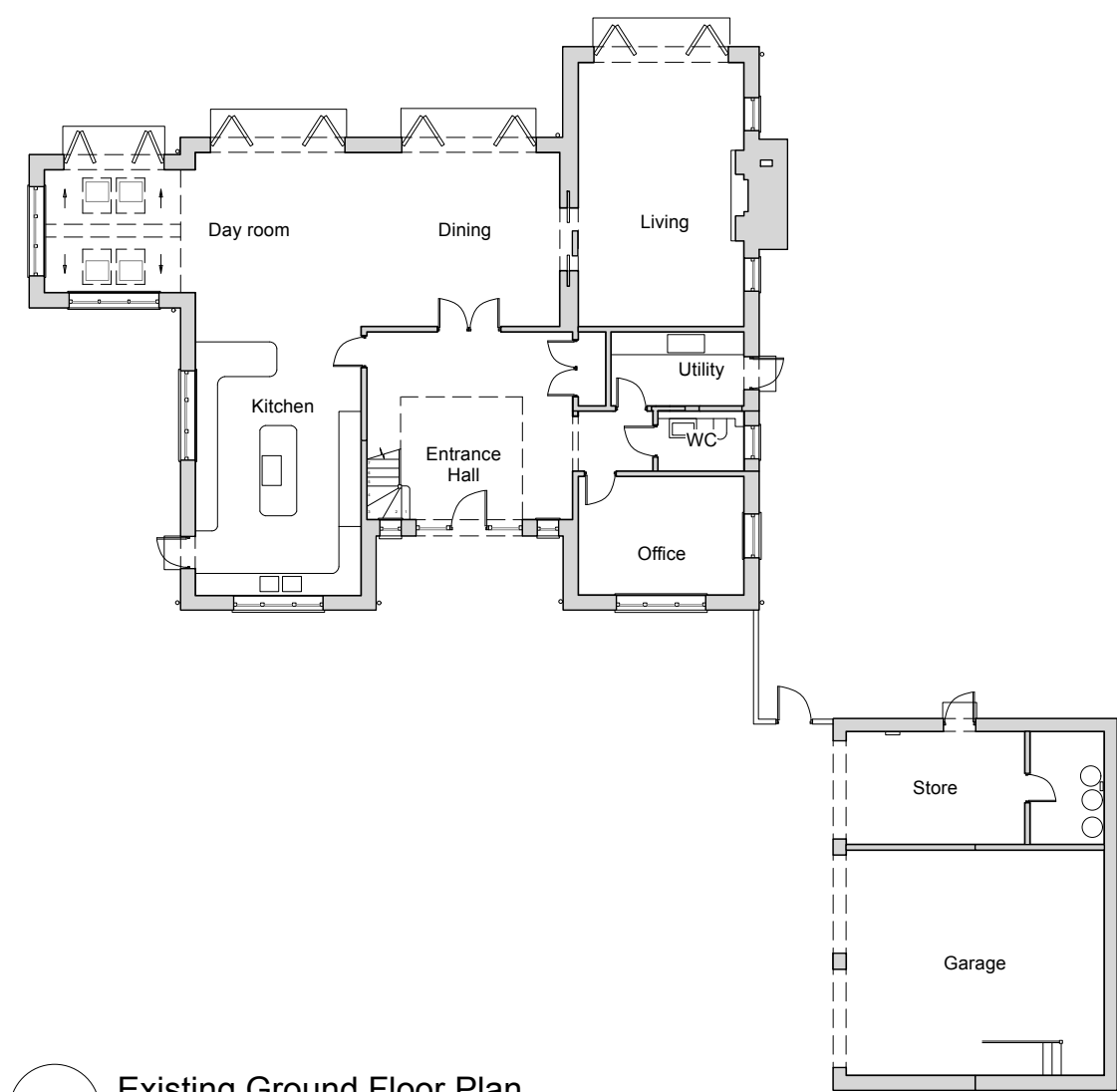
1 Existing Ground Floor Plan Scale: 1:200
