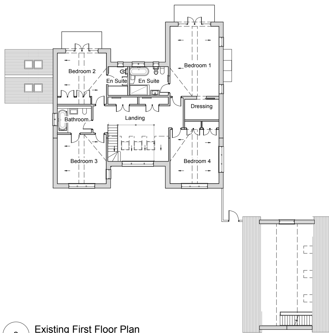
2 Existing First Floor Plan Scale: 1:200
