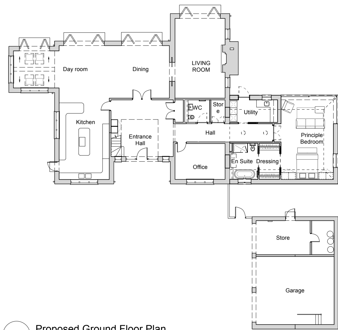
4 Proposed Ground Floor Plan Scale: 1:200
