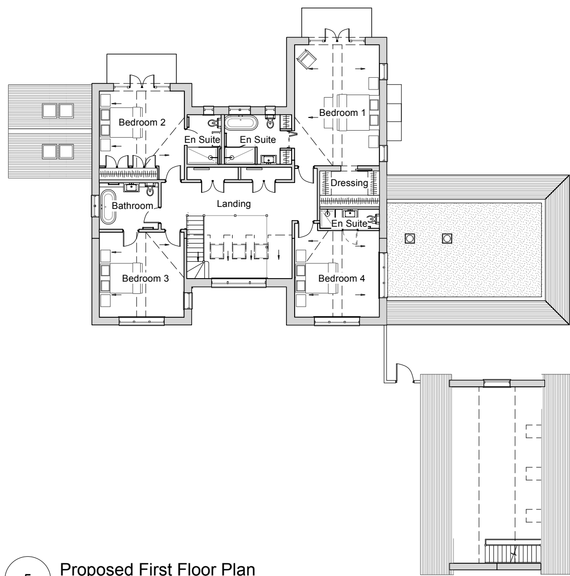
5 Proposed First Floor Plan Scale: 1:200
