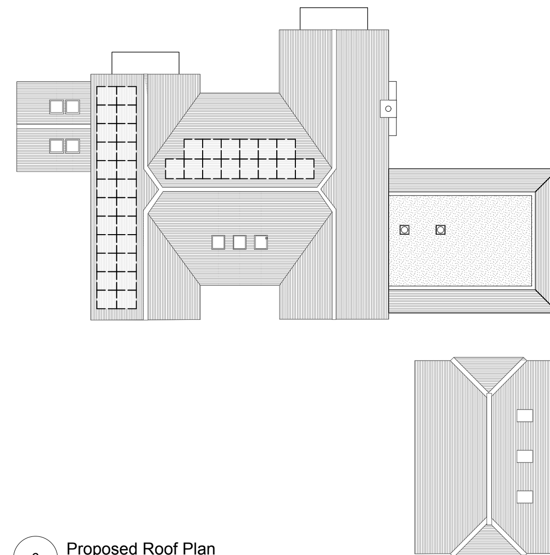
6 Proposed Roof Plan Scale: 1:200
