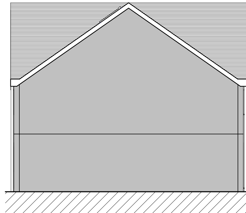
Proposed Side Elevation I 1 : 100
