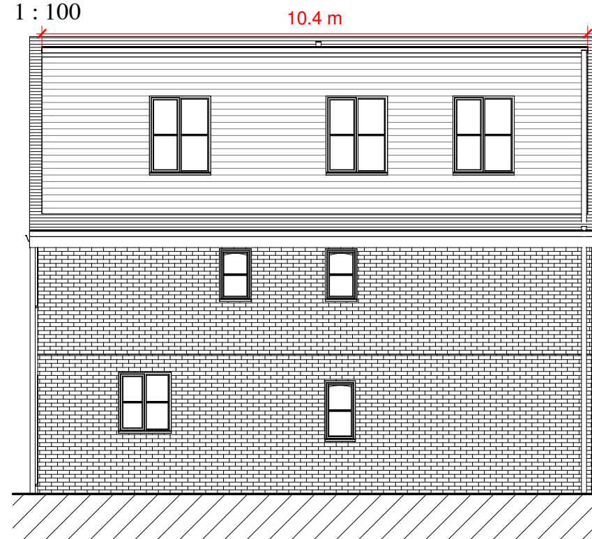
Proposed Side Elevation II 1 : 100
