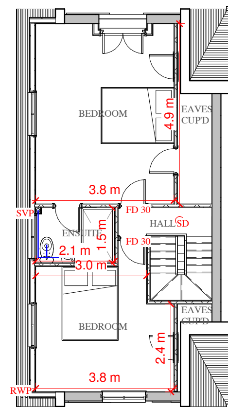
03 Proposed Second Floor 1 : 100
