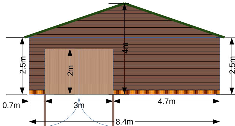
Rear Elevation: North
