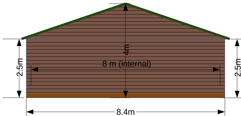
Rear Elevation: North
