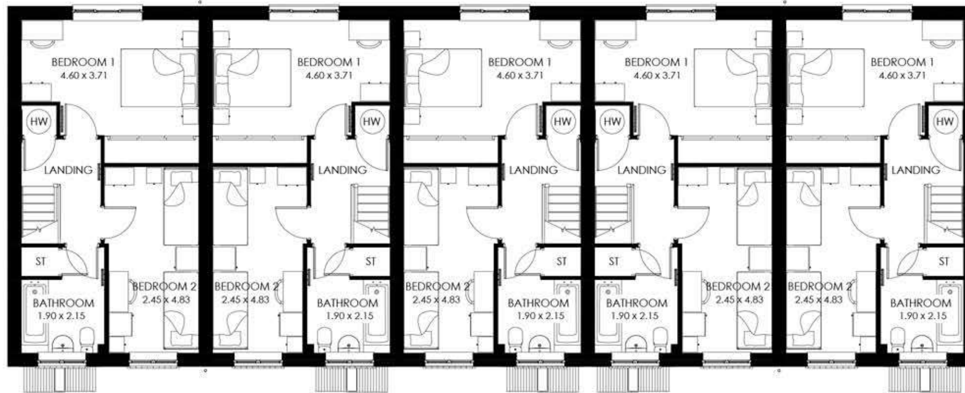
First Floor
