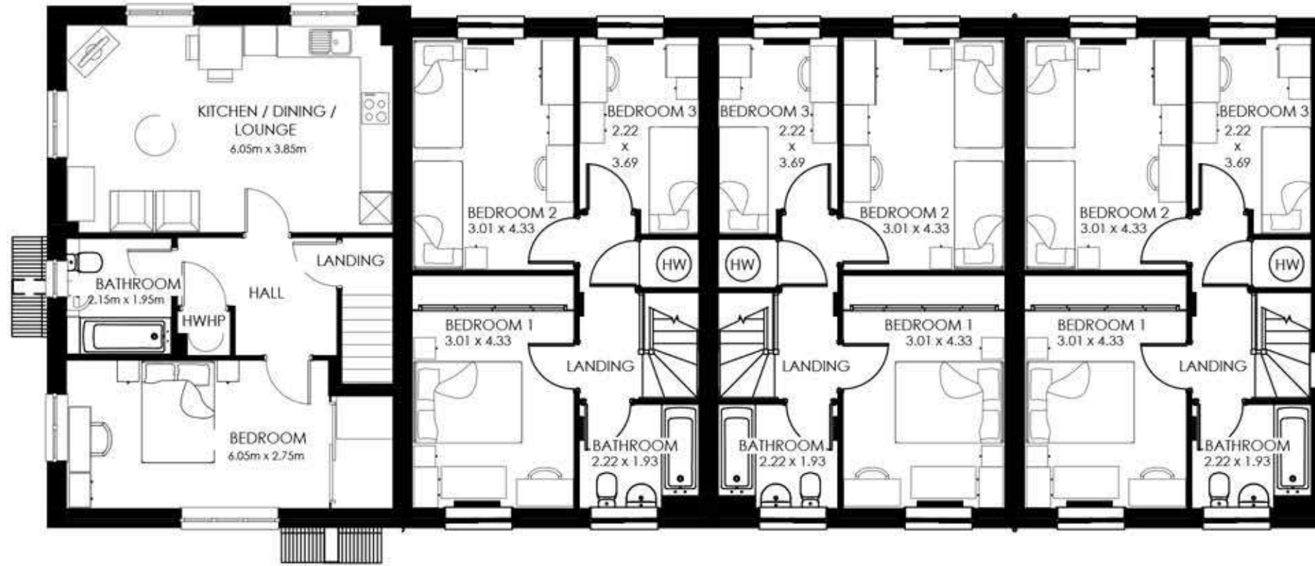
First Floor
