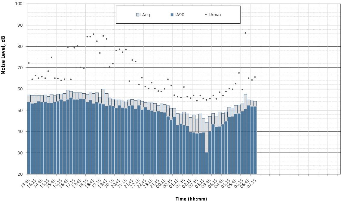
Horsham Employment Park ML2 Noise Time History Plot Thursday 6 November 2025
