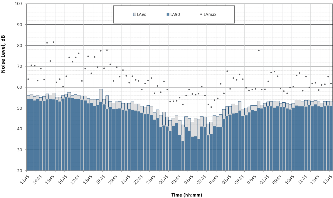
Horsham Employment Park ML2 Noise Time History Plot Saturday 8 November 2025
