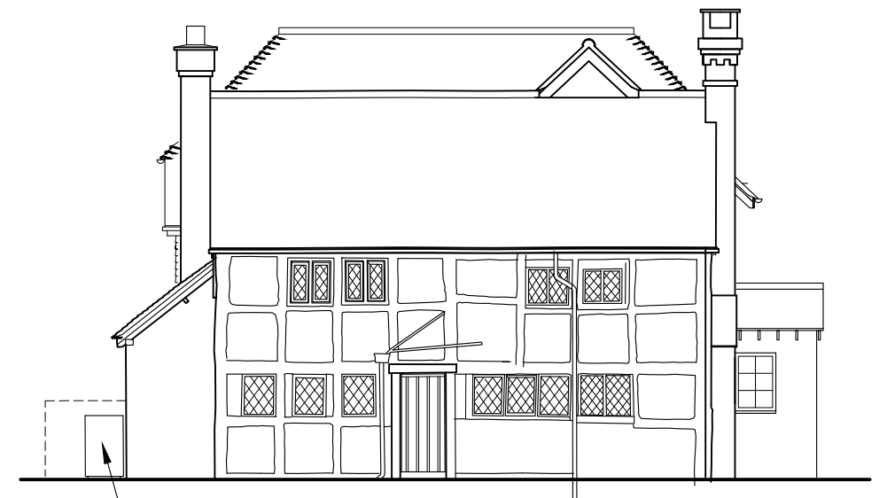
side elevation - faces west 1:100
