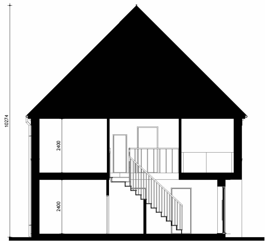
Building Section
