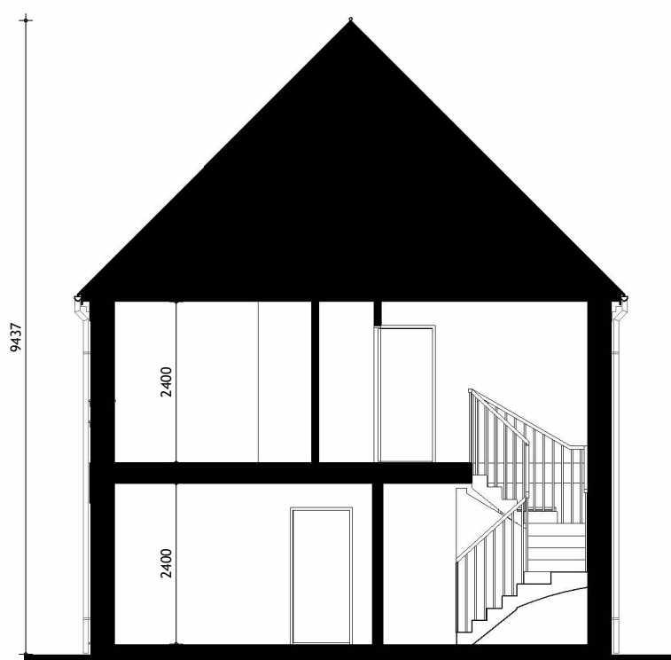
Building Section
