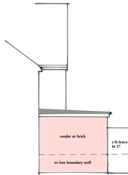
north elevation
