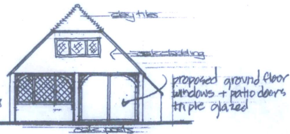
West elevation - proposed Elevations - scale: 1/100
