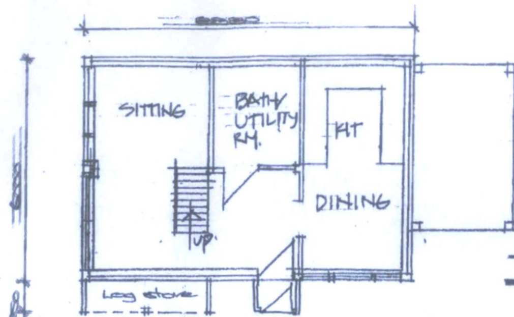
Ground Floor Plan - scale: 1/100 - proposed
