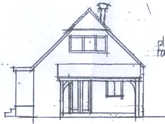
EAST ELEV-proposed 1:100
