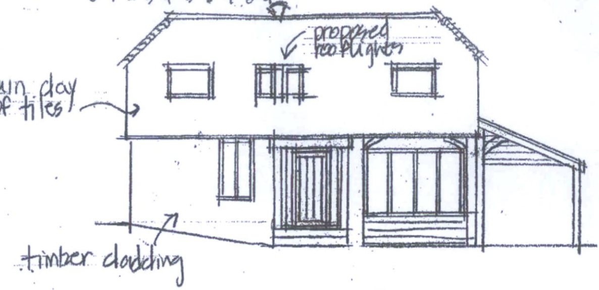
SOUTH elev - proposed 1:100
