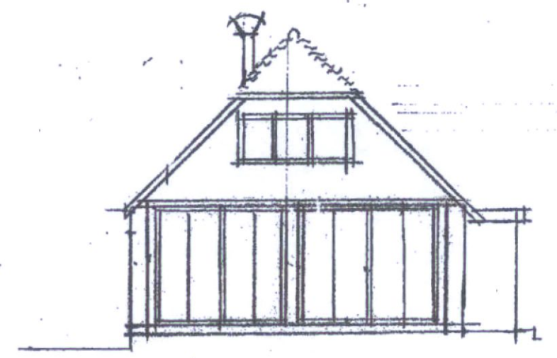
WEST ELEV -proposed 1:100
