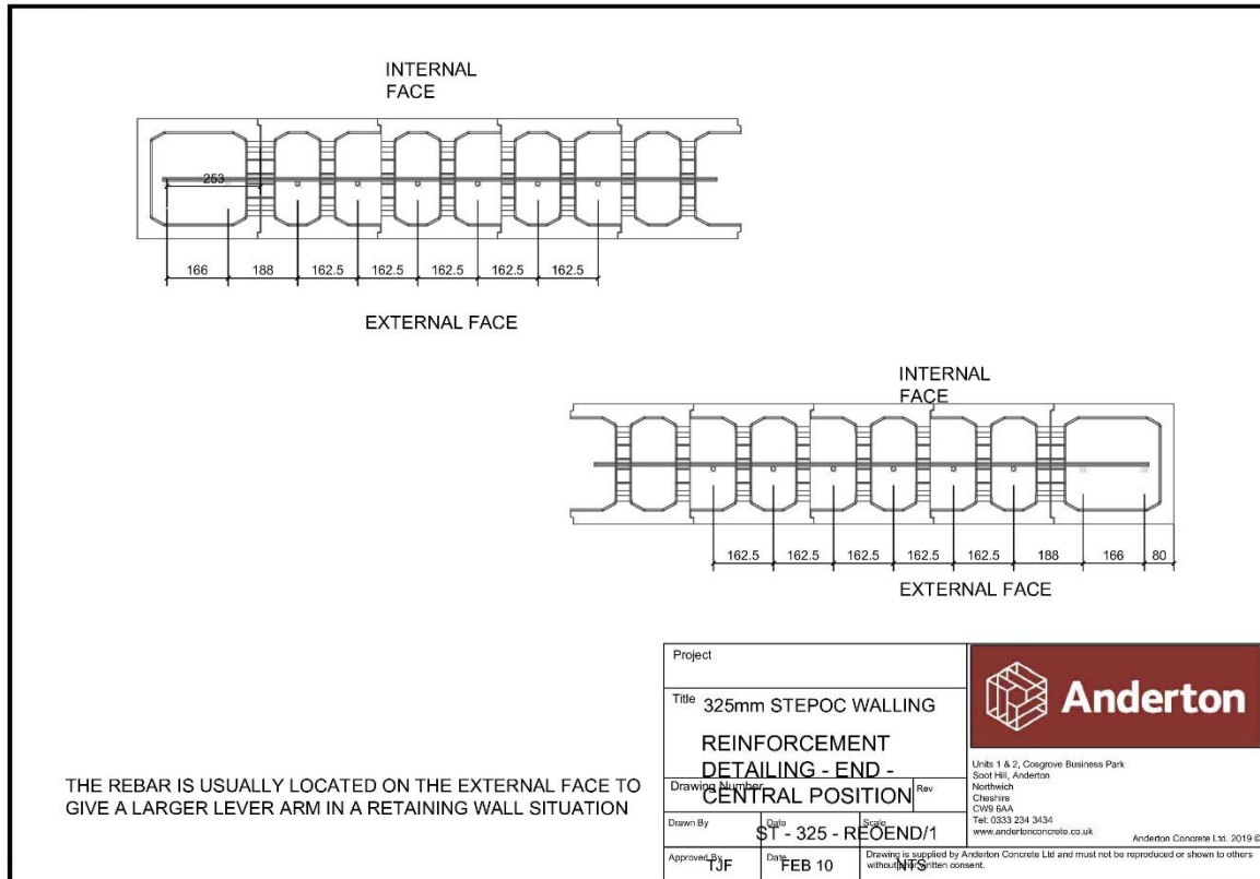
325mm Typical Stepoc Wall Construction
