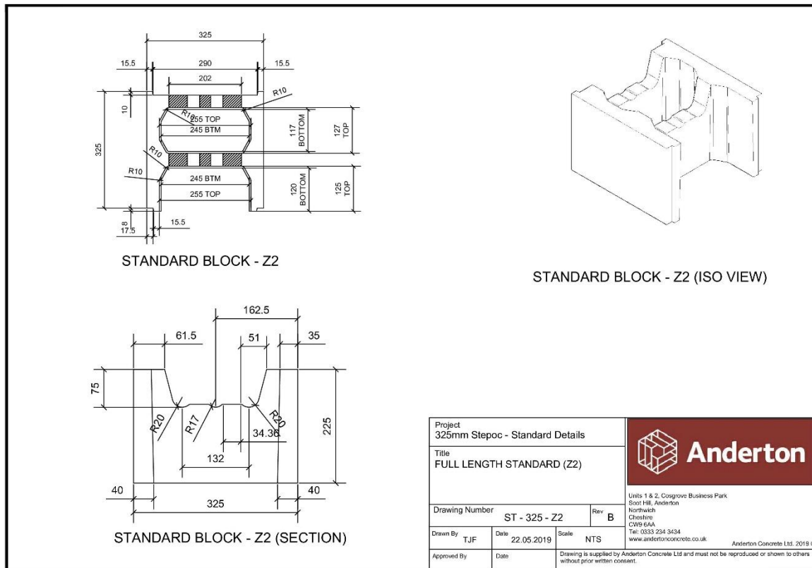
325mm Full Length Stepoc Block
