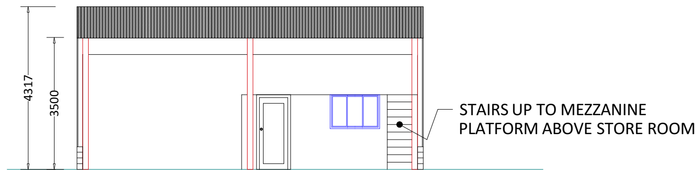
PRE-EXISTING EAST ELEVATION - (FRONT) 1:100 @ A1
