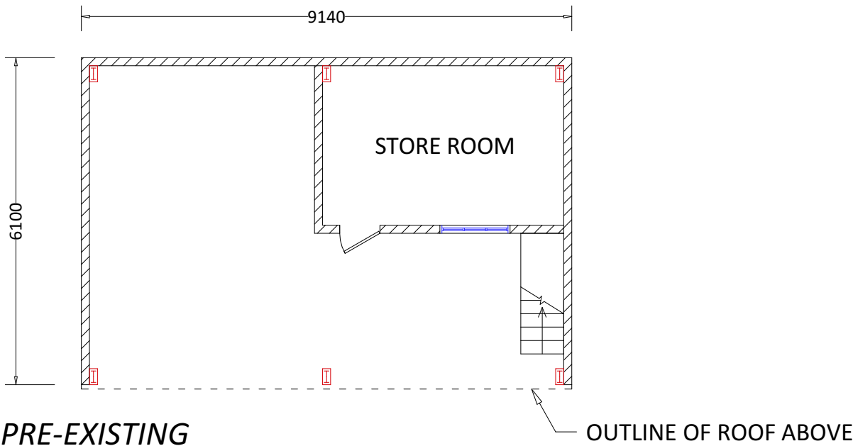
PRE-EXISTING BUILDING PLAN 1:100 @ A1
