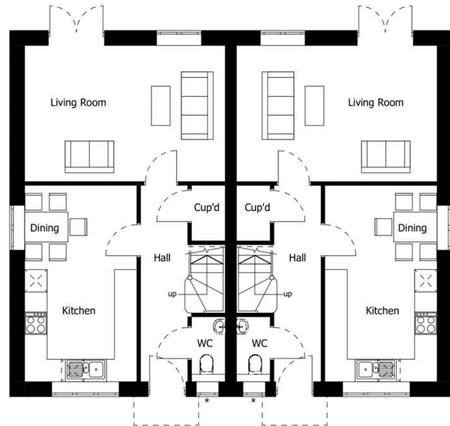
PROPOSED GROUND FLOOR [1:100]
