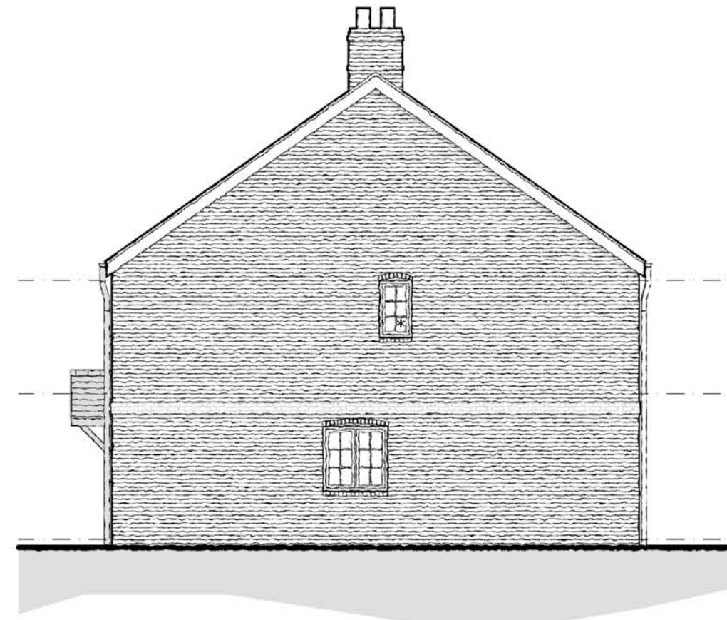
PROPOSED SIDE ELEVATION [1] [1:100]
