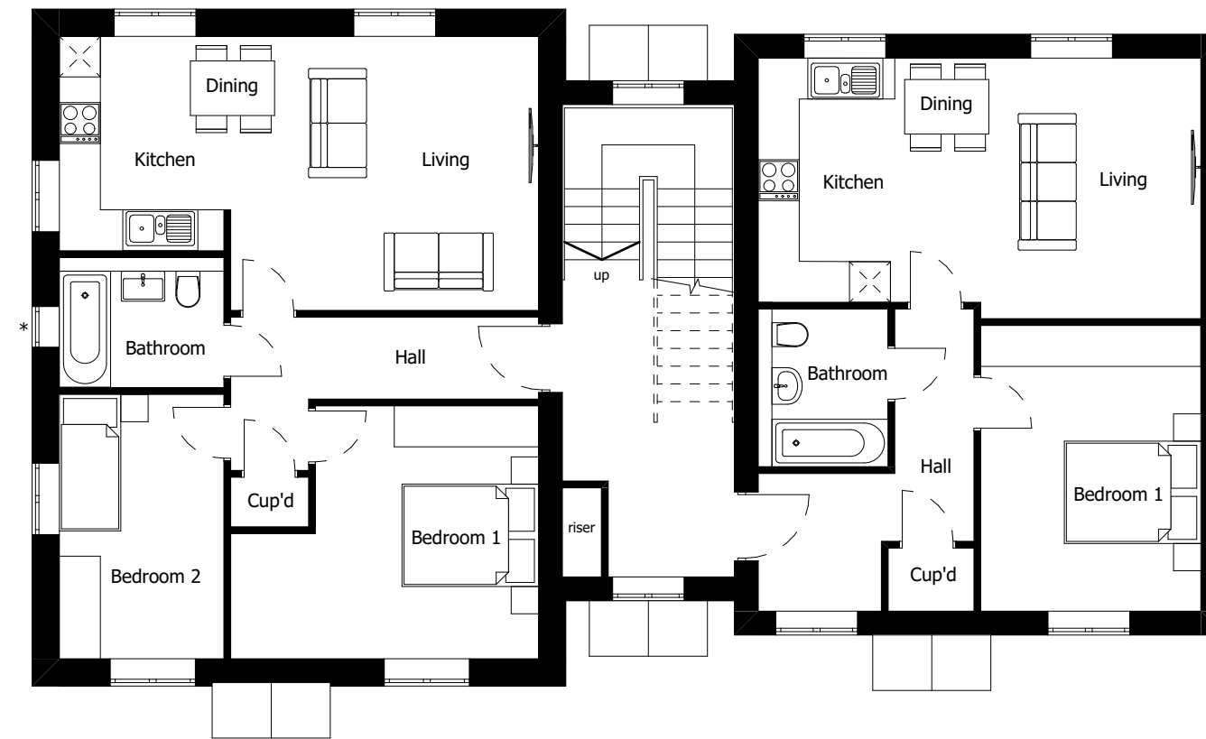
PROPOSED FIRST FLOOR [1:100]
