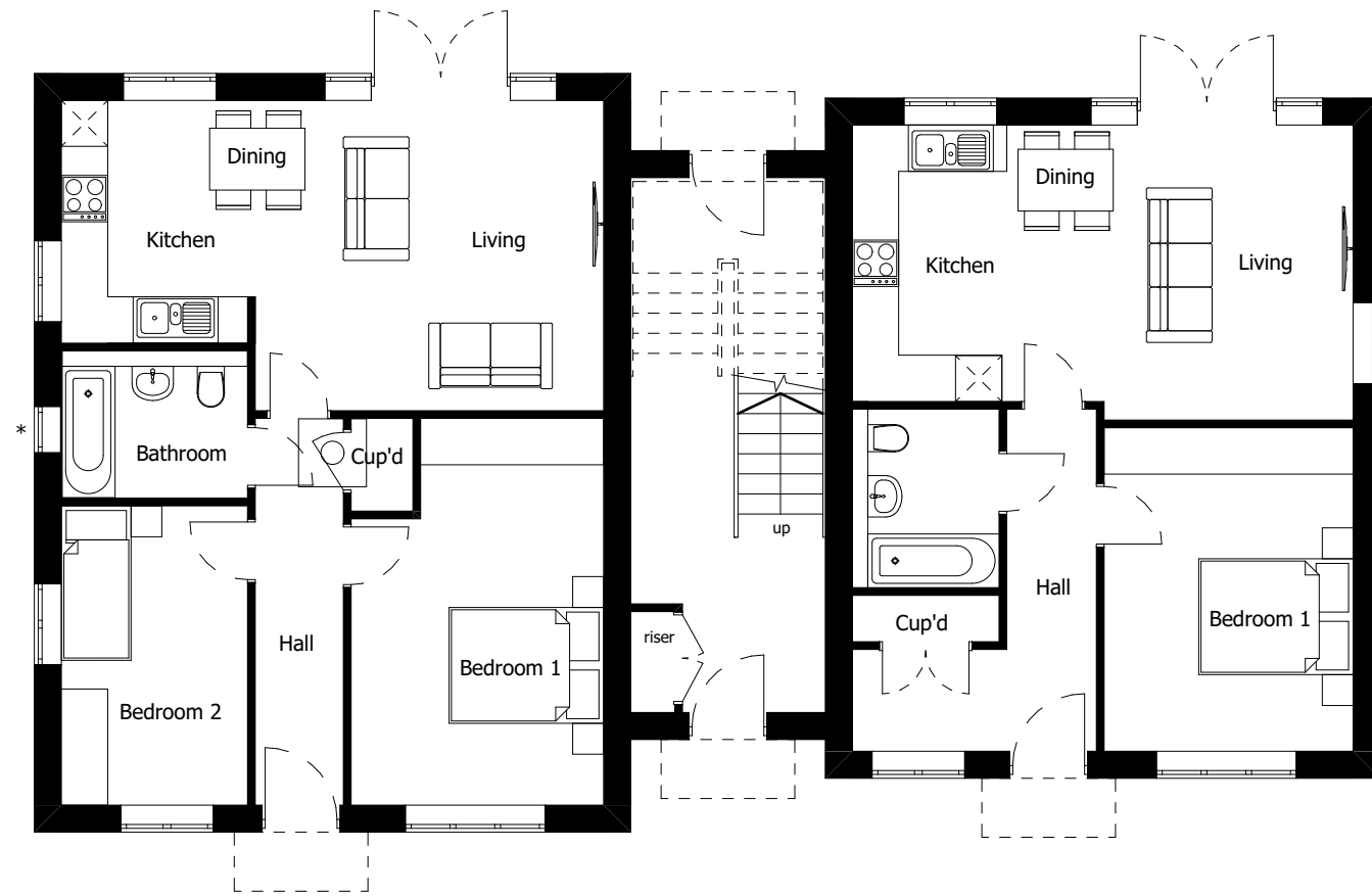
PROPOSED GROUND FLOOR [1:100]
