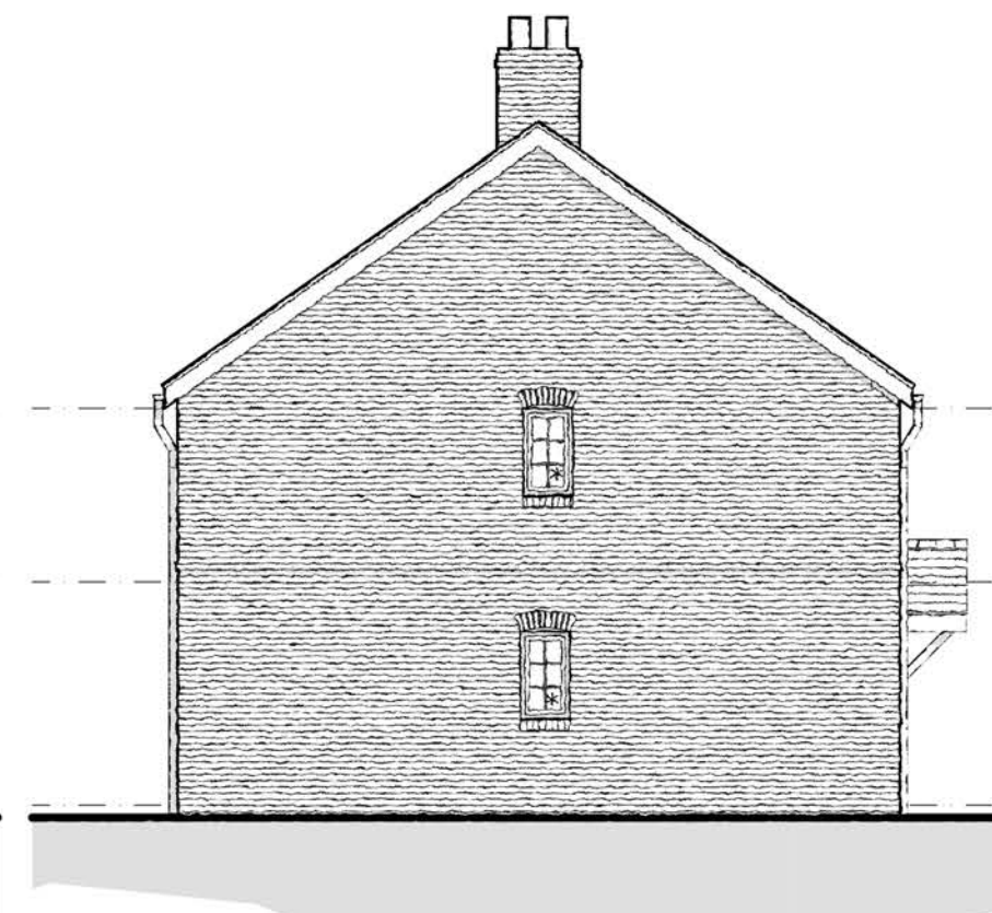
PROPOSED SIDE ELEVATION [2] [1:100]
