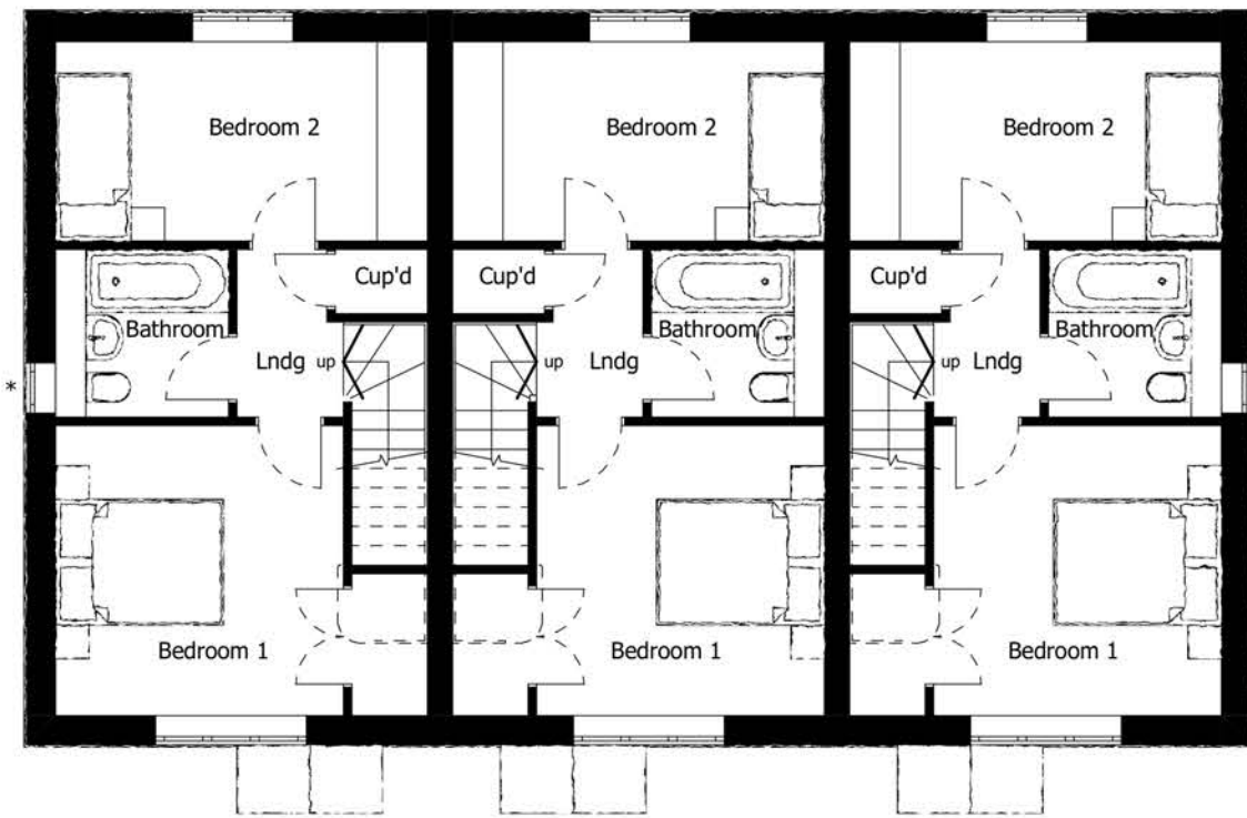
PROPOSED FIRST FLOOR [1:100]
