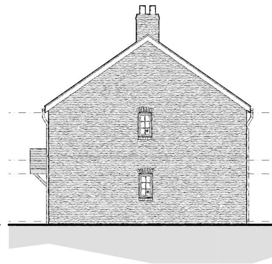
PROPOSED SIDE ELEVATION [1] [1:100]
