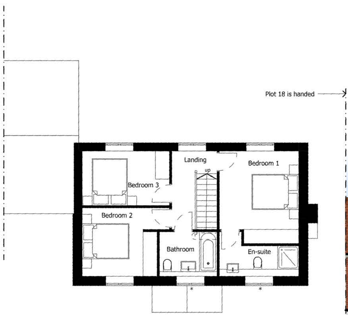
PROPOSED FIRST FLOOR [1:100]
