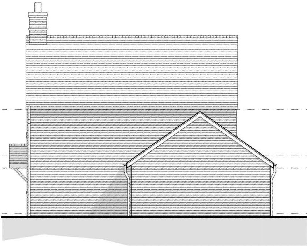
PROPOSED SIDE ELEVATION [1] [1:100]
