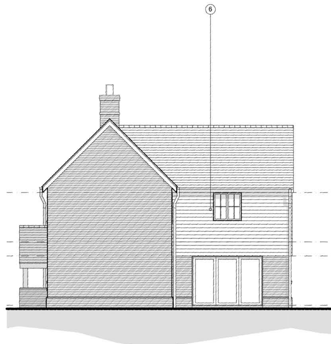
PROPOSED SIDE ELEVATION [1] [1:100]
