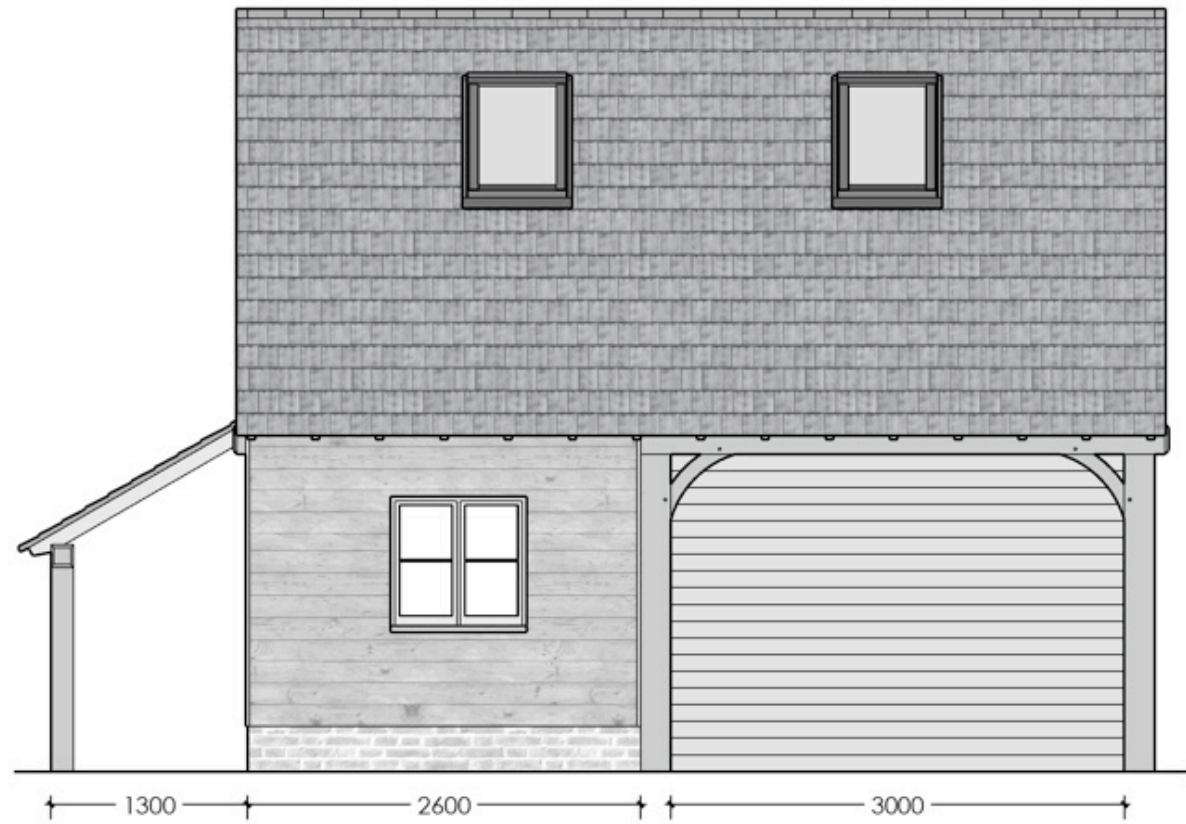
Front Elevation
