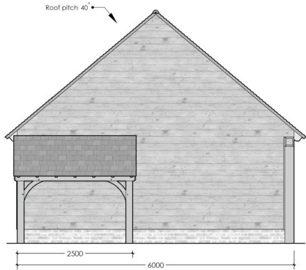
Left Elevation
