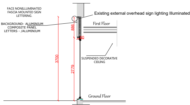
PROPOSED SIGN SECTION A-A
