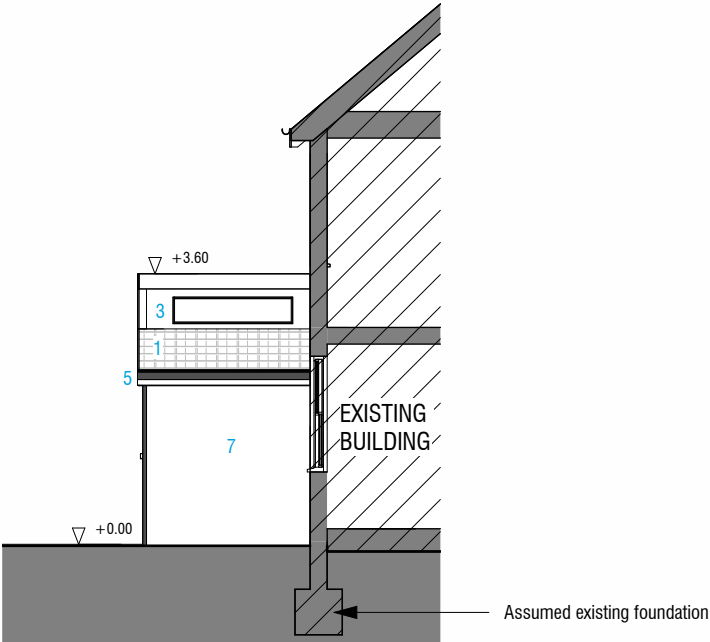
4 SHORT SIDE ELEVATION 1 : 100
