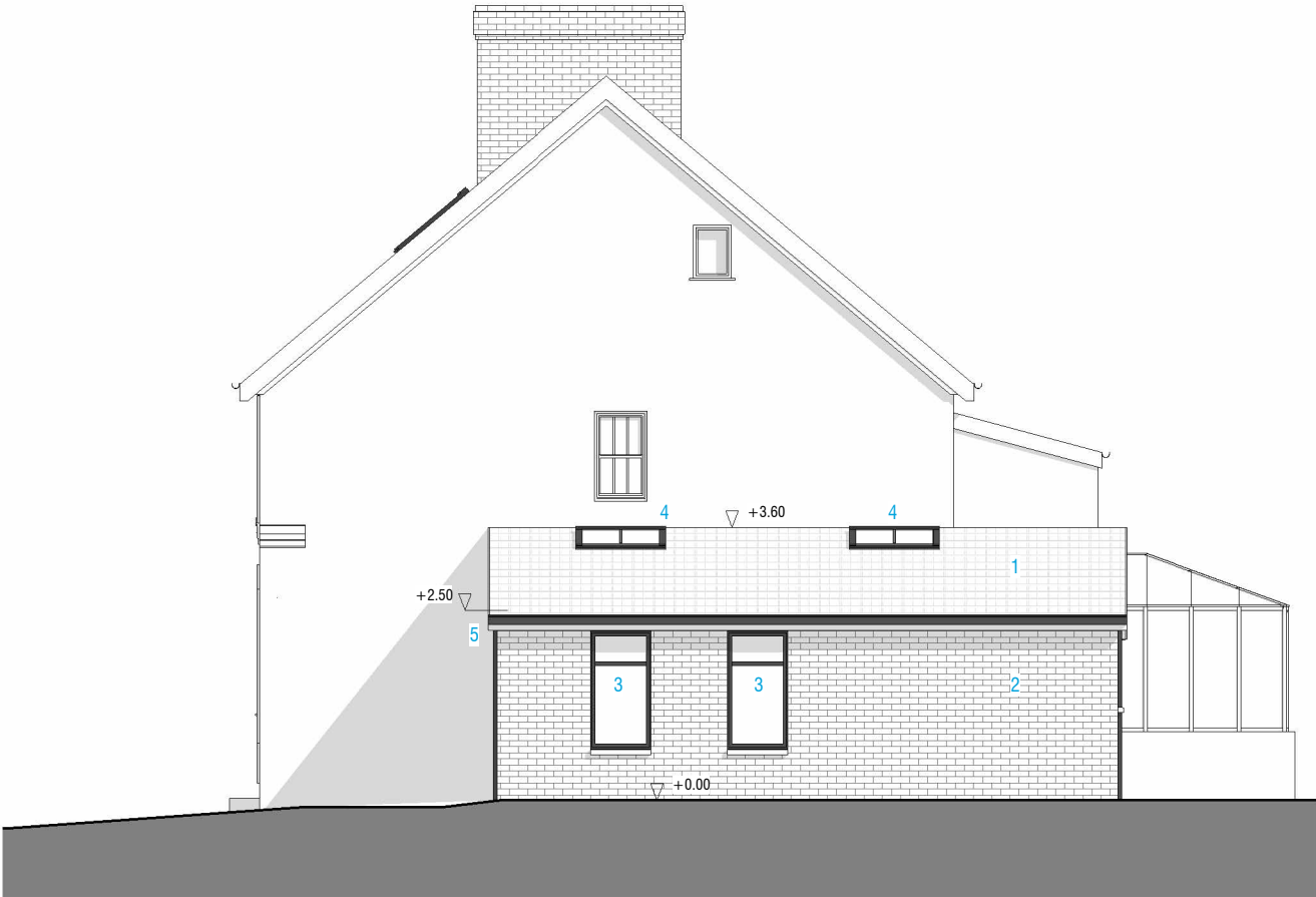
1 SIDE ELEVATION 1 : 100
