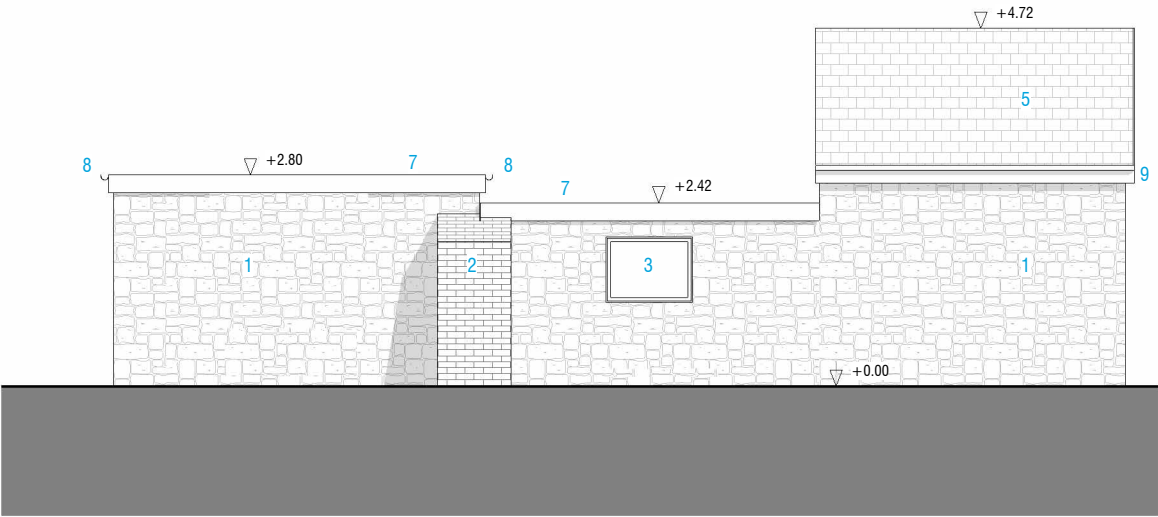
1 OUTBUILDING - WEST ELEVATION 1 : 100
