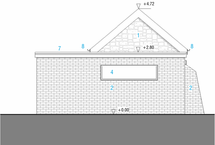
4 OUTBUILDING- NORTH ELEVATION 1 : 100
