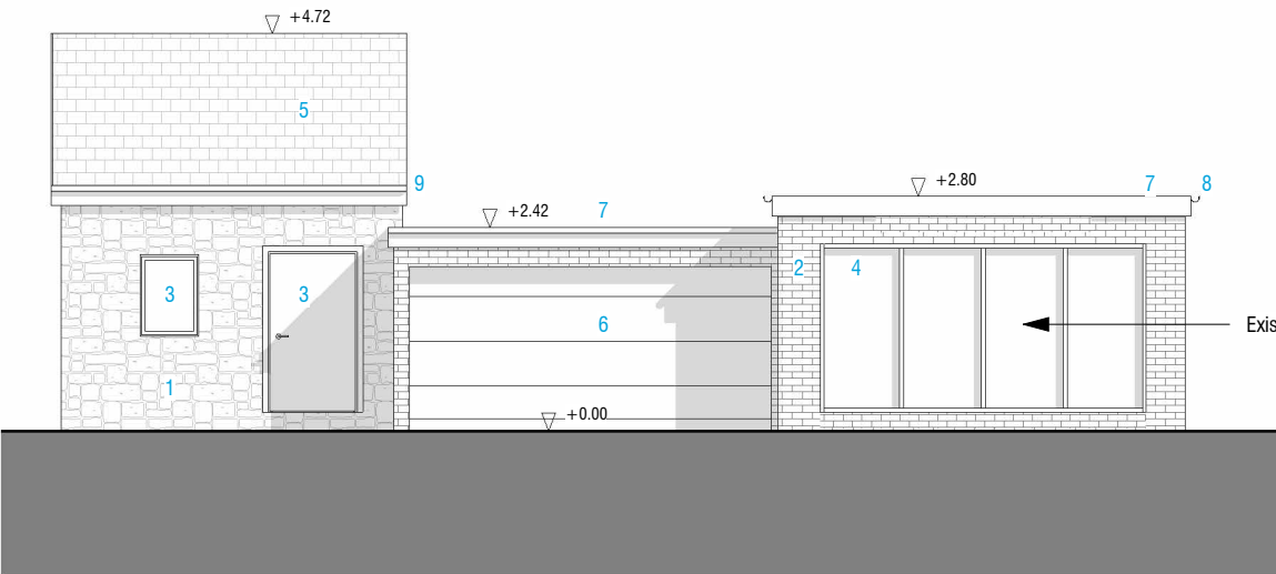
2 OUTBUILDING - EAST ELEVATION 1 : 100
