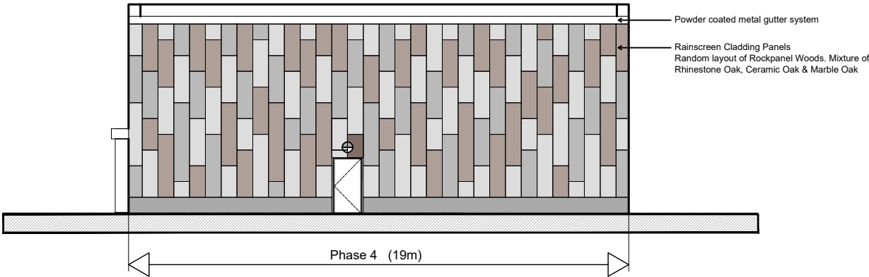
Northern Elevation
