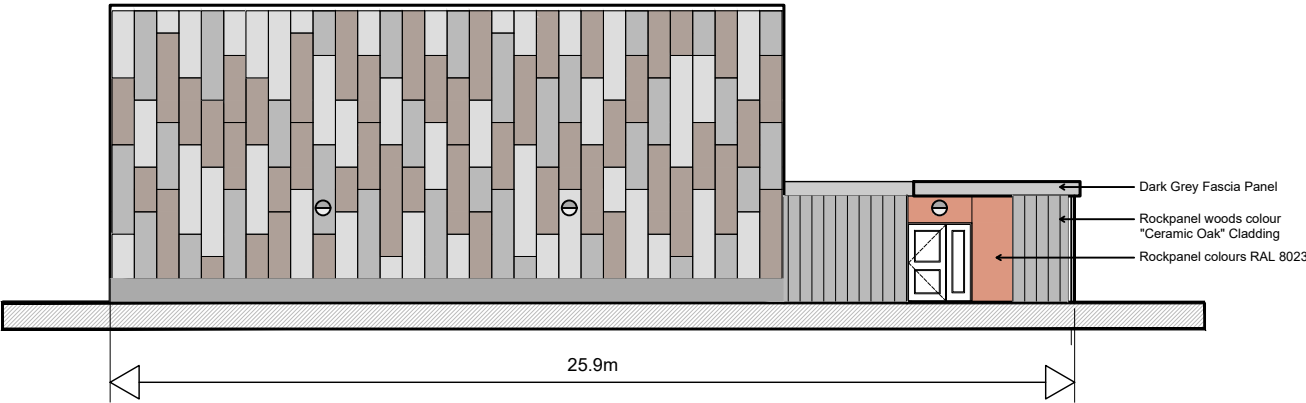
Western Elevation
