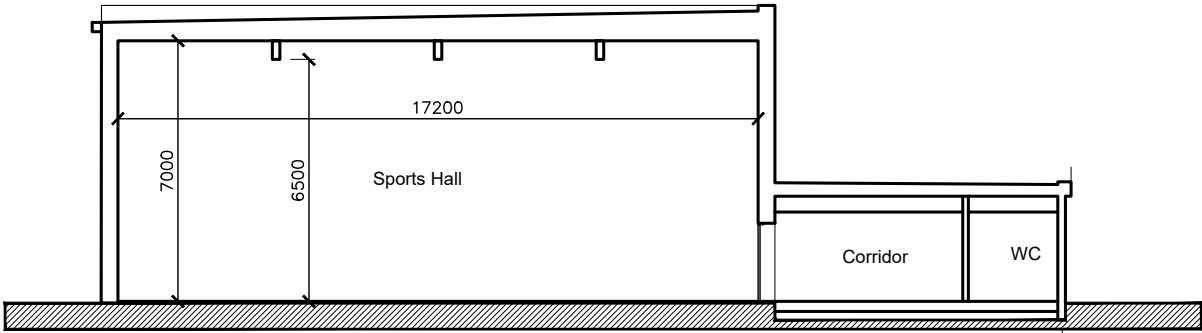
Cross Section
