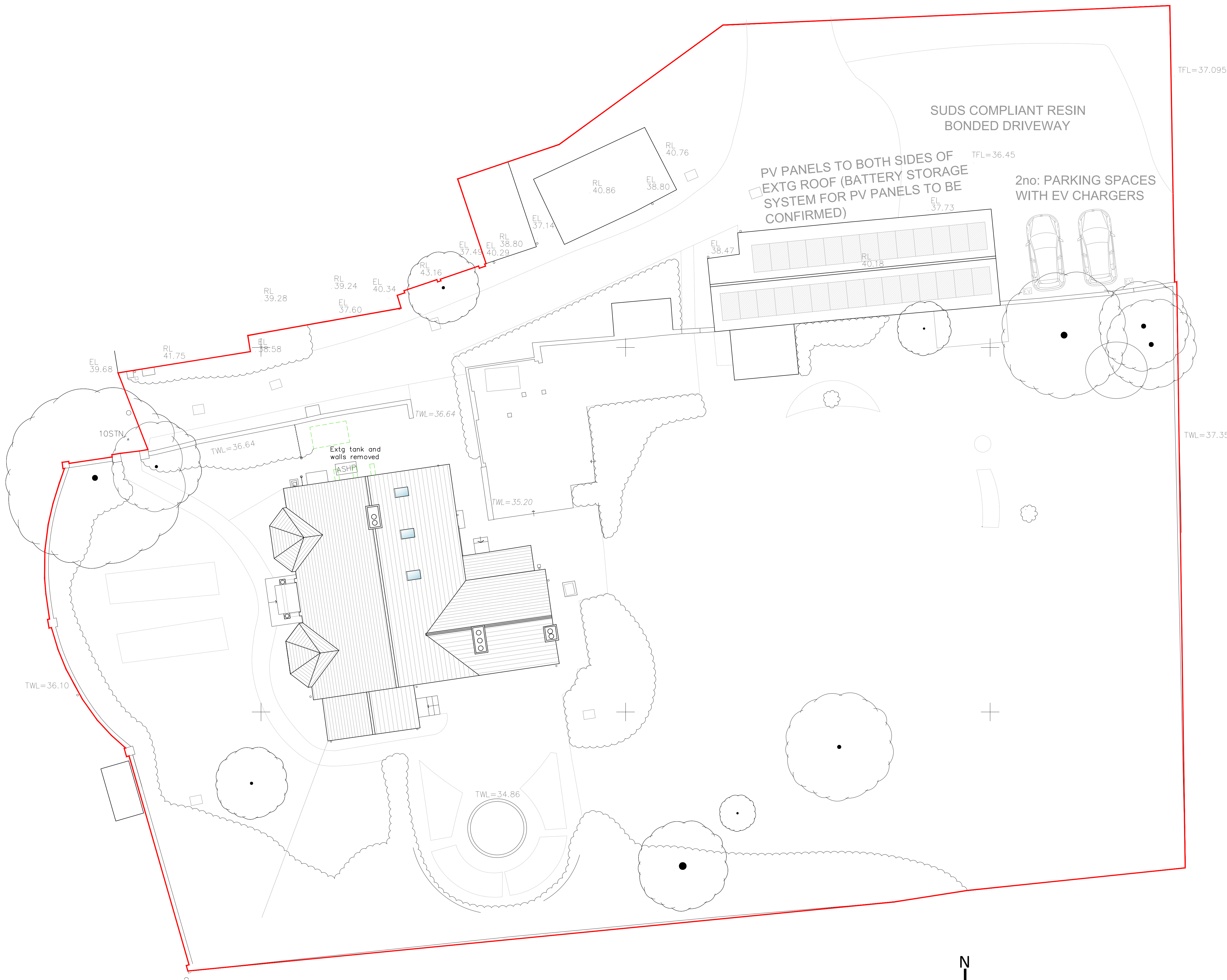
PROPOSED SITE LAYOUT 1:100
