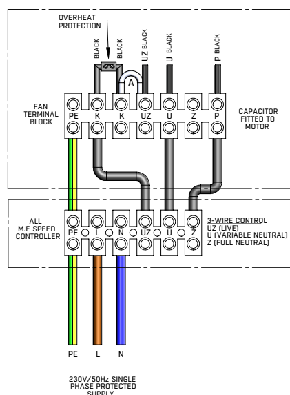
FAN CONNECTED TO SPEED CONTROLLER (VARIABLE SPEED)
