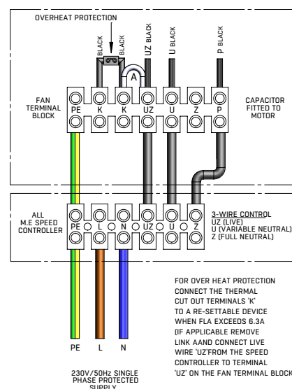
FAN CONNECTED TO SPEED CONTROLLER (VARIABLE SPEED)
