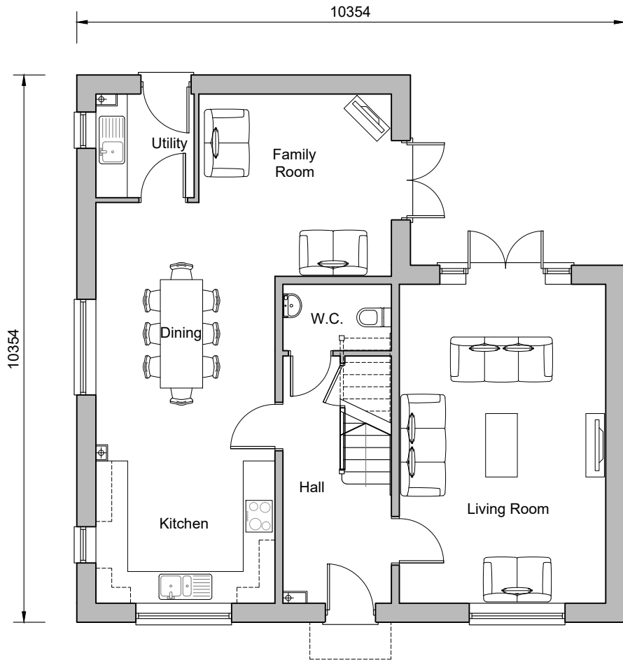
Ground Floor Plan Plot 56
