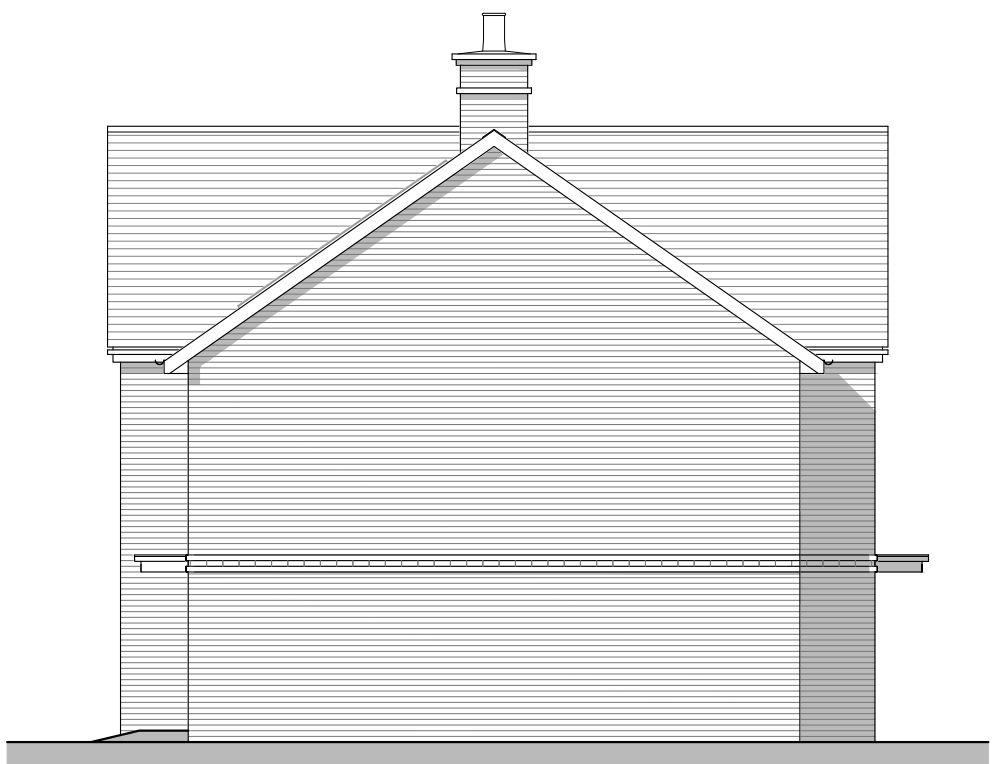
Side Elevation
