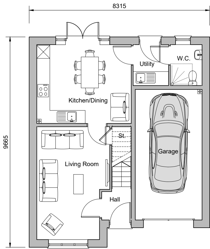
Ground Floor Plan Plots 251
