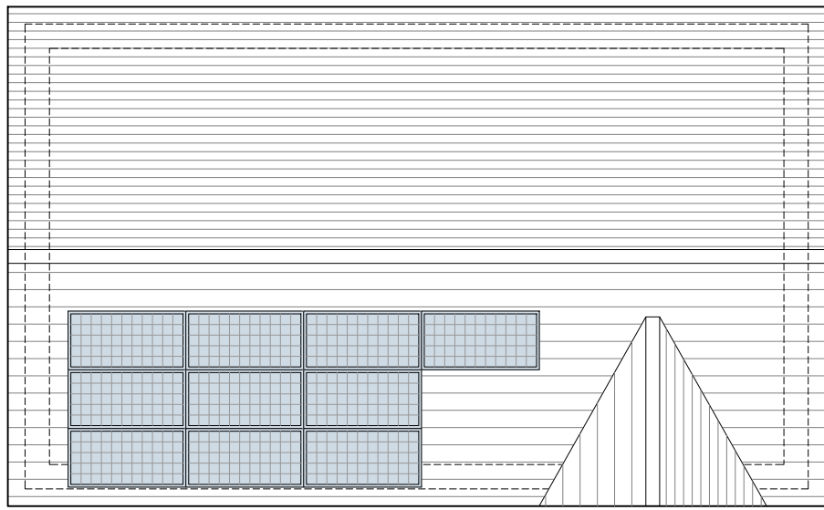
Roof Plan
