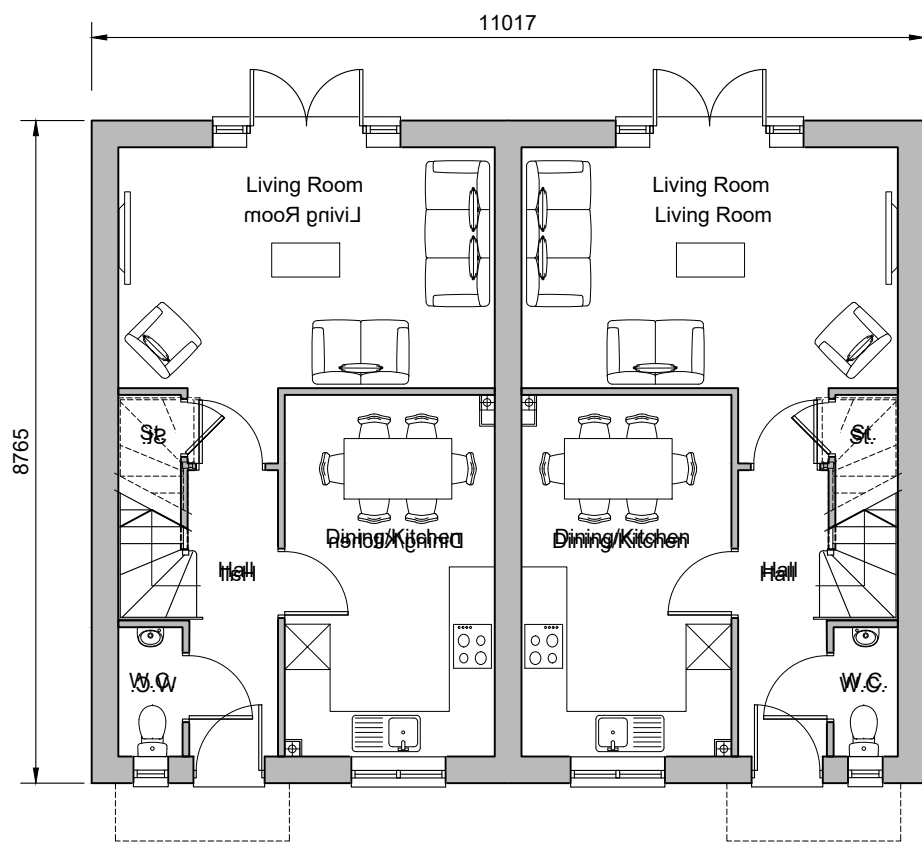
Ground Floor Plan Plots 175-176
