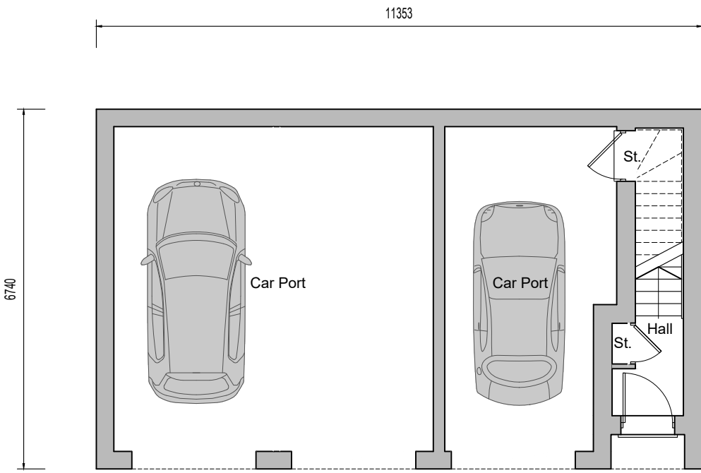
Ground Floor Plan Plot 167
