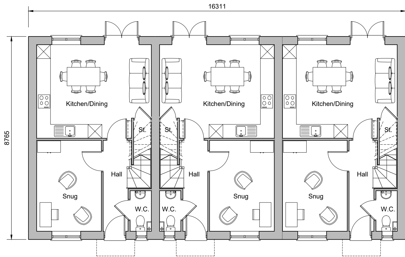
Ground Floor Plan Plots 144-146, 256-258, 261-263
