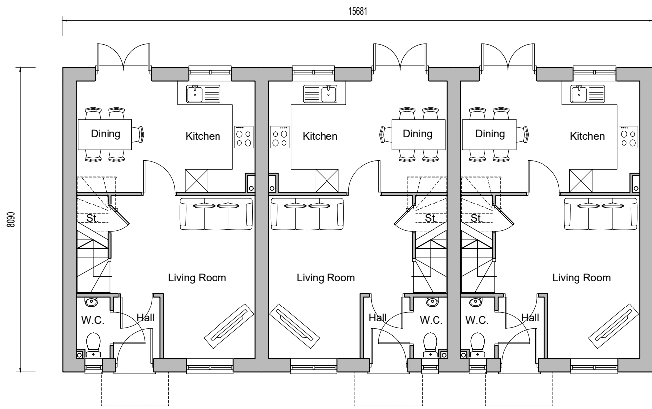
Ground Floor Plan Plots 124-126, 180-182
