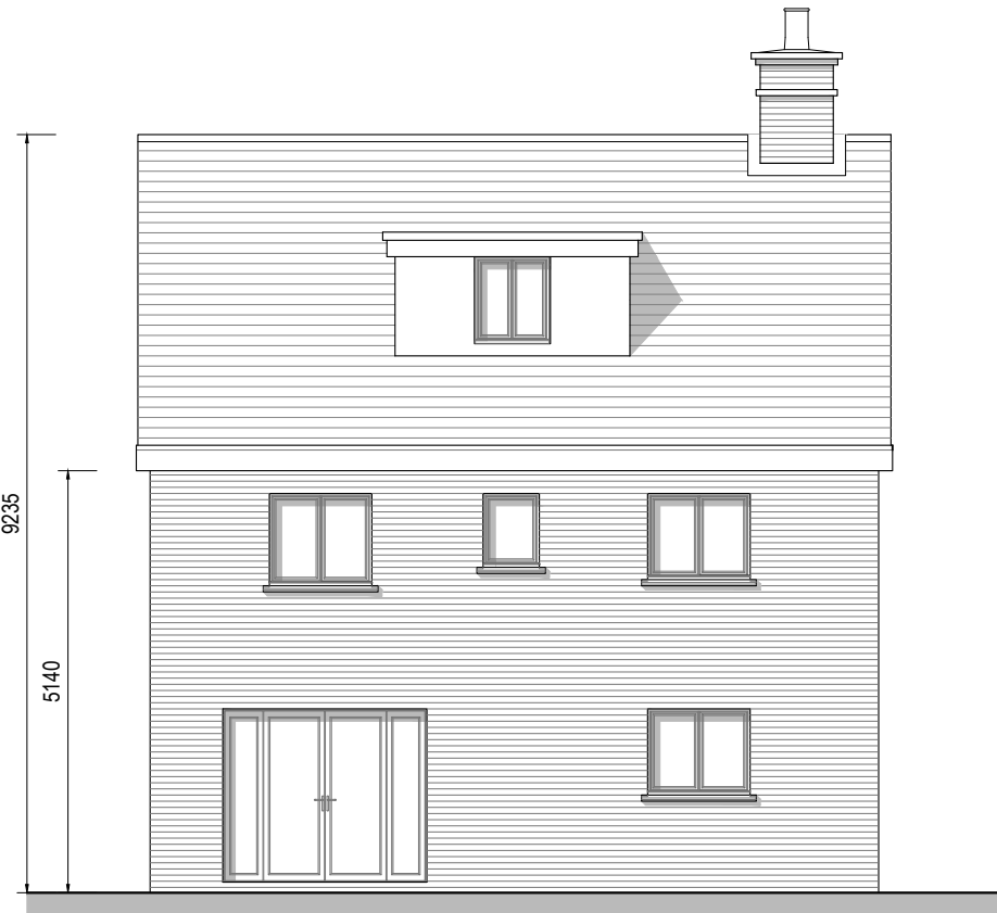
Rear Elevation Chimney to plots 40, 152, 205 only
