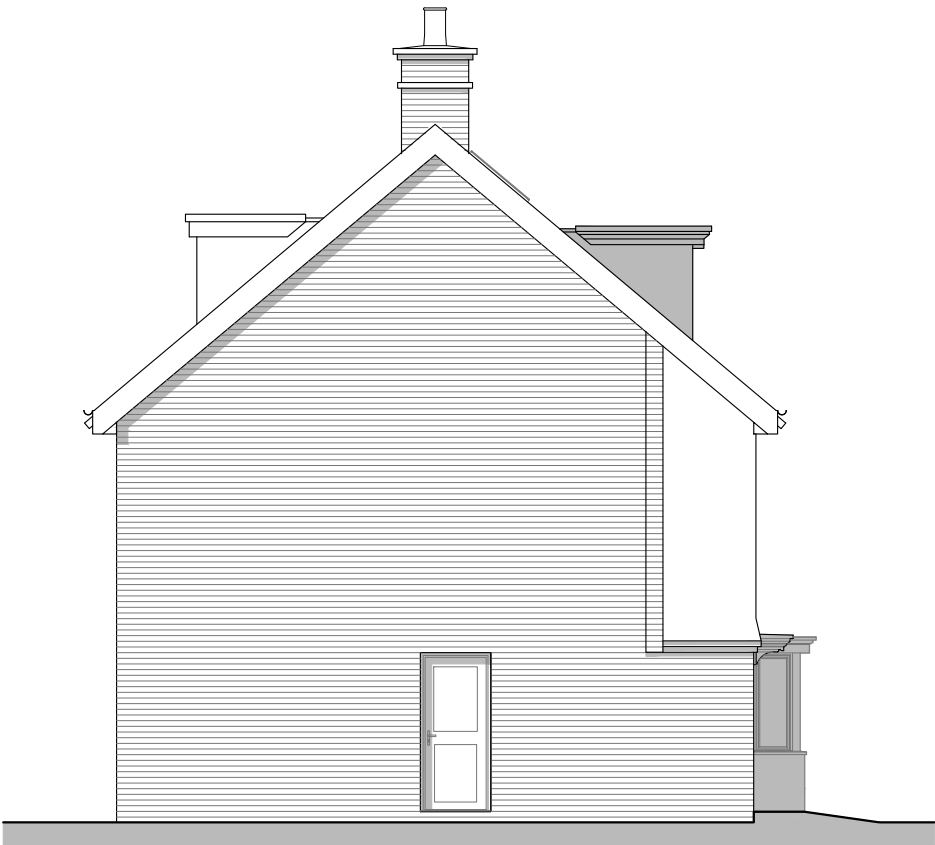
Side Elevation
