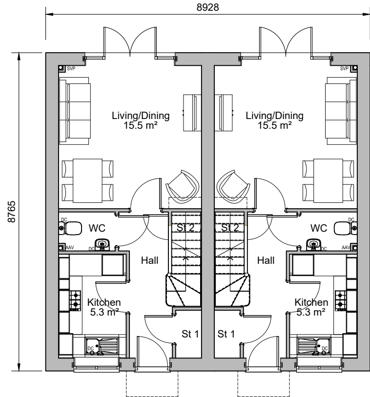
Ground Floor Plan Plots 115-116, 130-131
