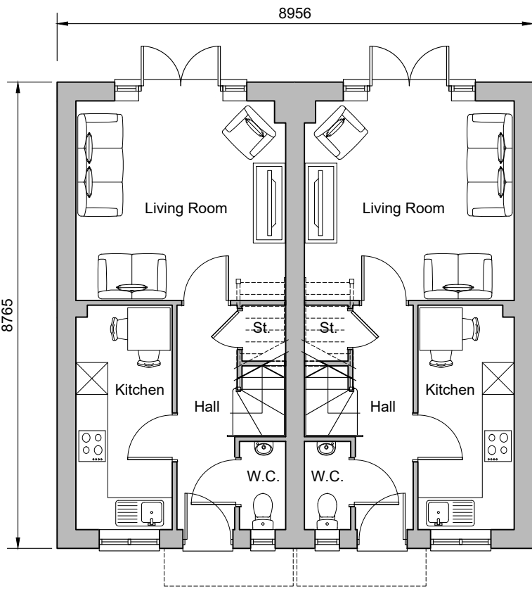
Ground Floor Plan Plots 113-114
