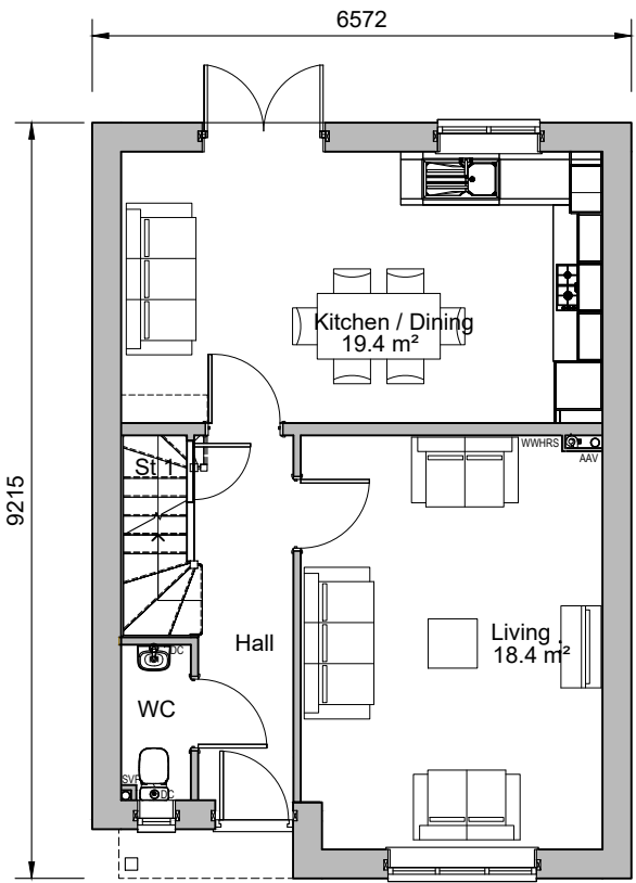
Ground Floor Plan Plot 249 Plots 103 and 121 (handed)
