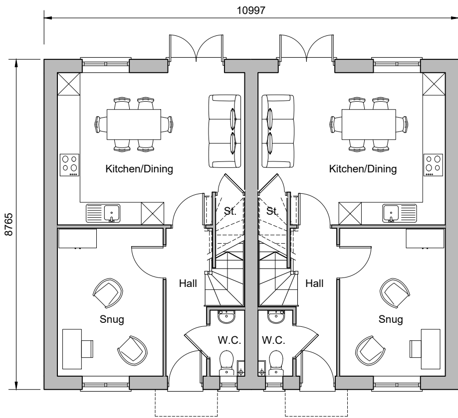
Ground Floor Plan Plots 99-100 and 215-216
