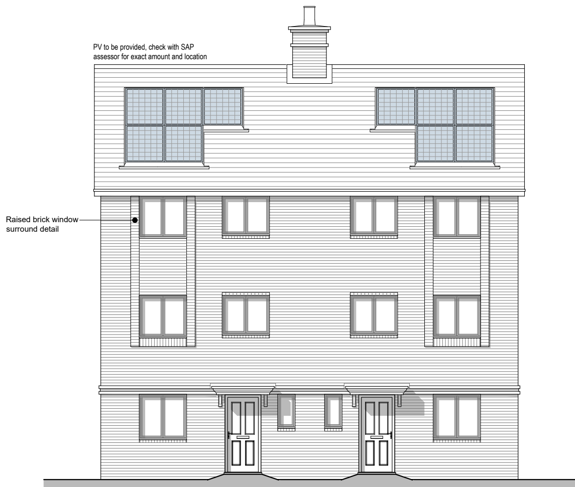
Front Elevation
