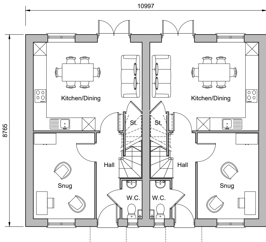
Ground Floor Plan Plots 90-91
