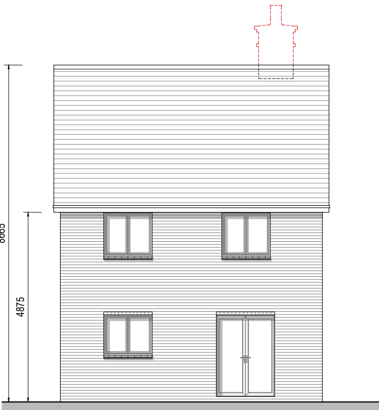
Rear Elevation Chimney (shown dotted) to Plot 95 only
