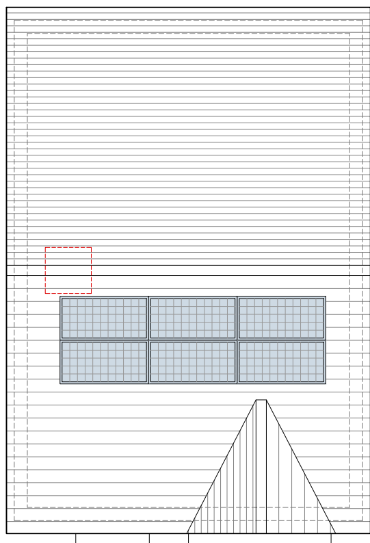
Roof Plan Chimney (shown dotted) to Plot 95 only
