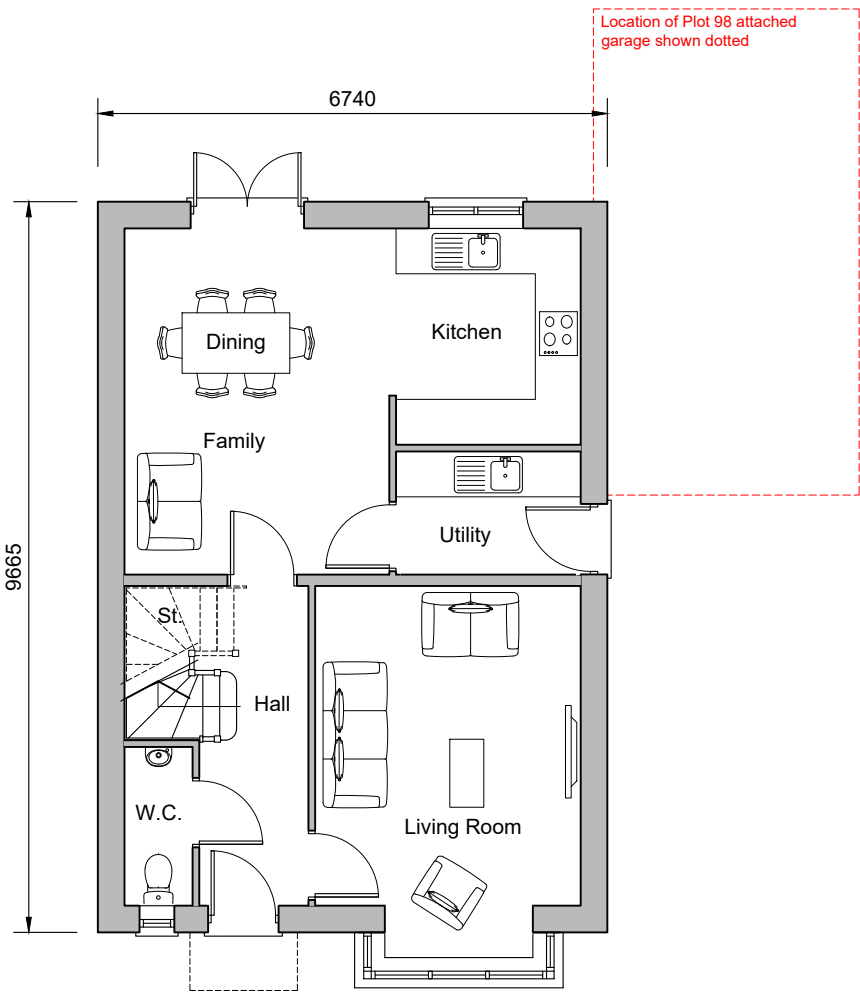
Ground Floor Plan Plots 72, 94, 95, 98, 108, 109, 110, 159, 199, 232, 233 Plots 101, 158 (handed).
