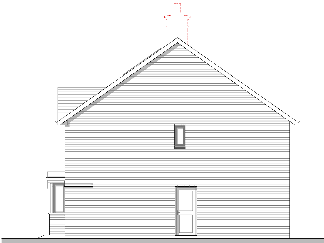
Side Elevation Chimney (shown dotted) to Plot 95 only
