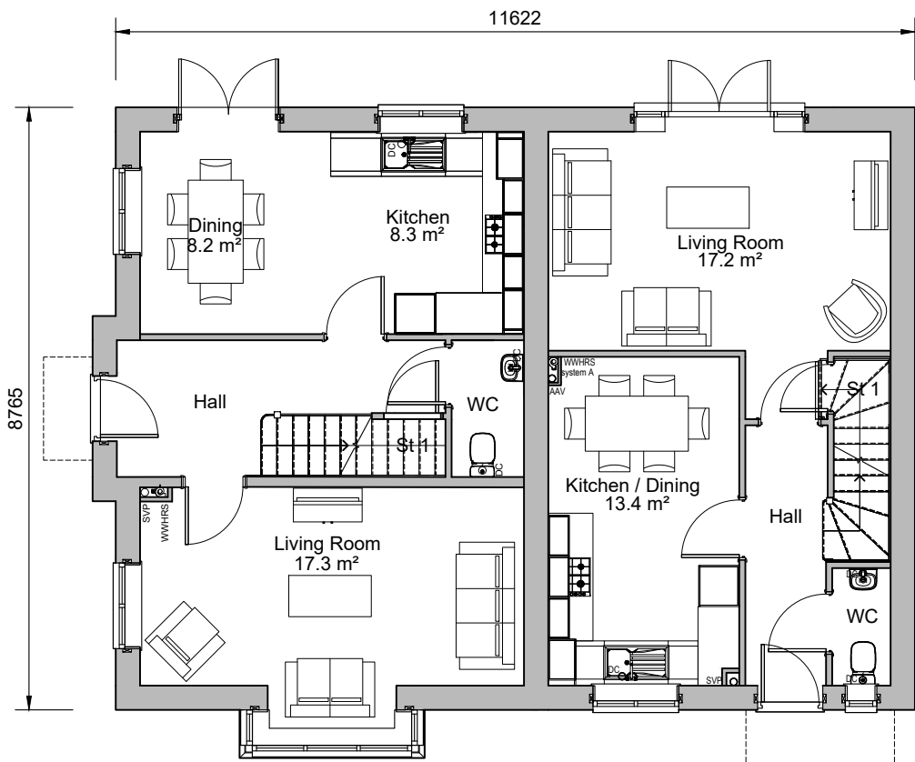
Ground Floor Plan Plots 50-51, 73-74
