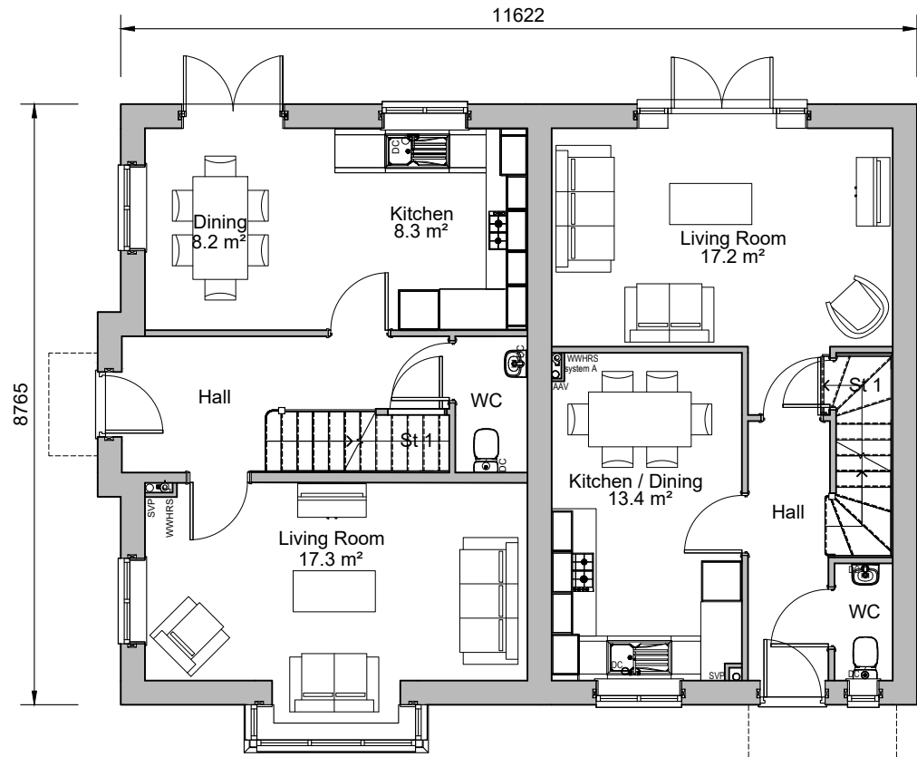
Ground Floor Plan Plots 111-112, 160-161, 234-235 and 273-274 Plots 44-45, 186-187, 202-203, 246-247, 264-265 and 268-269 (handed)
