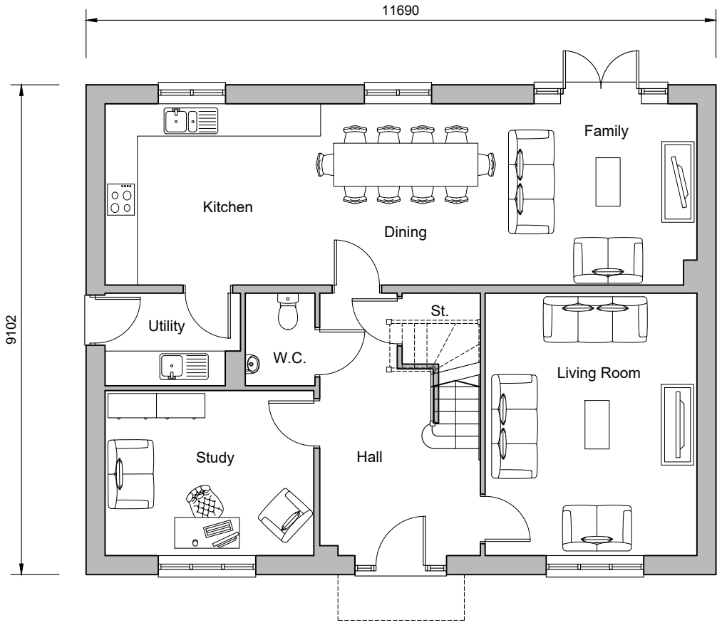
Ground Floor Plan Plot 42
