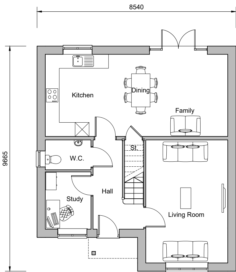
Ground Floor Plan Plots 41 and 96
