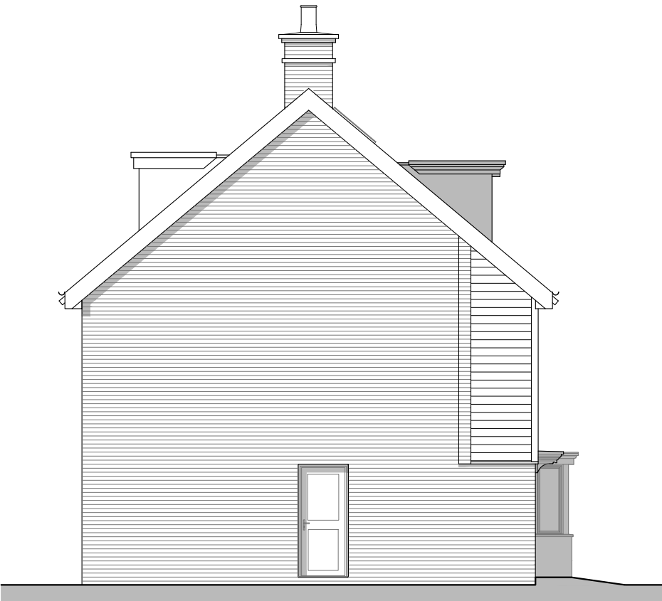
Side Elevation
