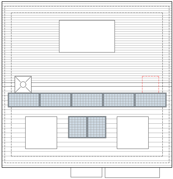
Roof Plan Chimney to plots 39, 43 only Chimney shown dotted to plots 53, 54 only
