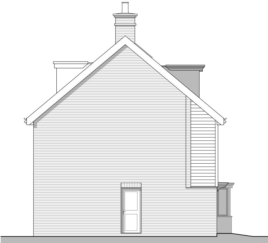
Side Elevation Plot 43 only
