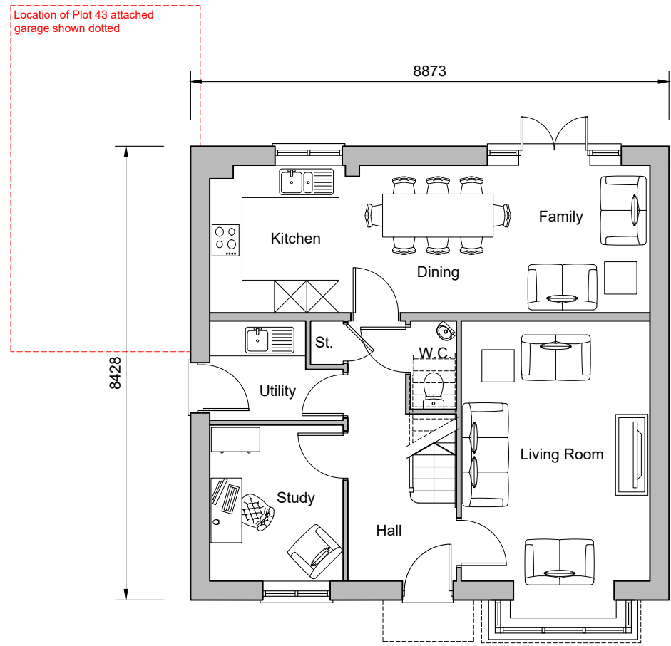
Ground Floor Plan Plots 39, 43, 53, 69 Plots 54, 55, 70 (handed)
