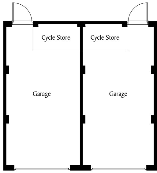
Garage Floor Plans - Plots 165-166, 218-219,
